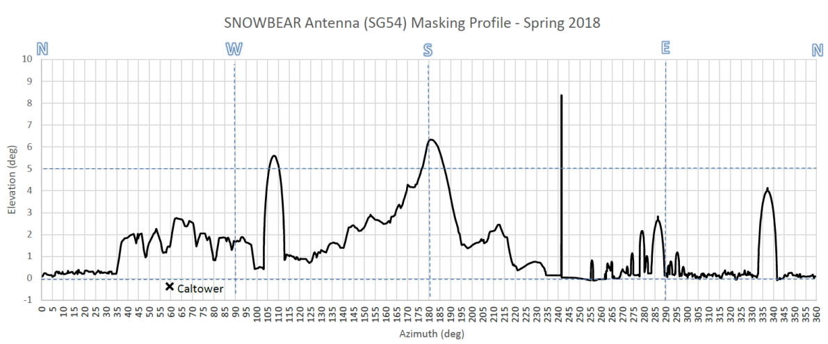
Figure F-1. SNOWBEAR Horizon Mask
