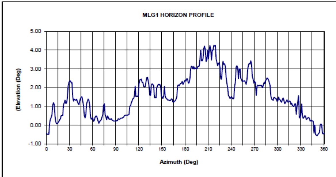
Figure F-3. Malargüe Horizon Mask
