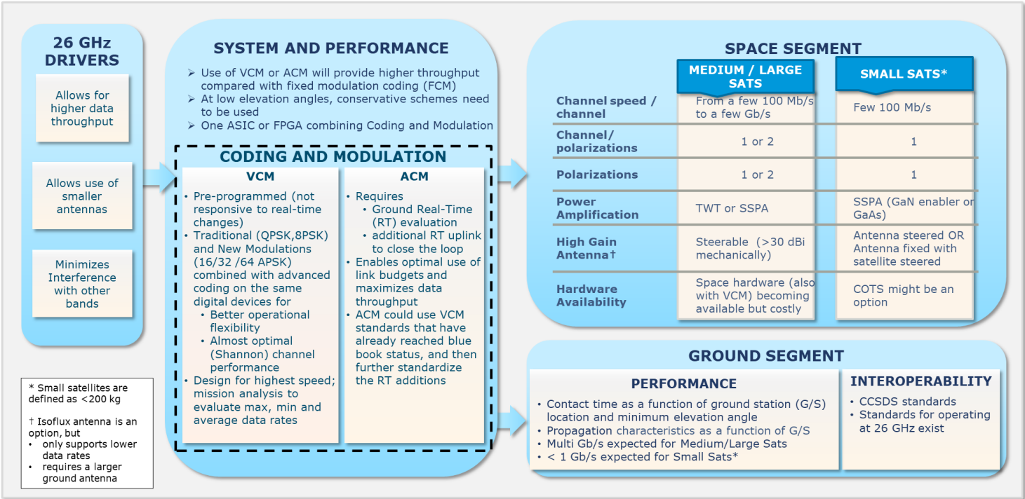
Figure J-1. 26 GHz Decision Checklist
