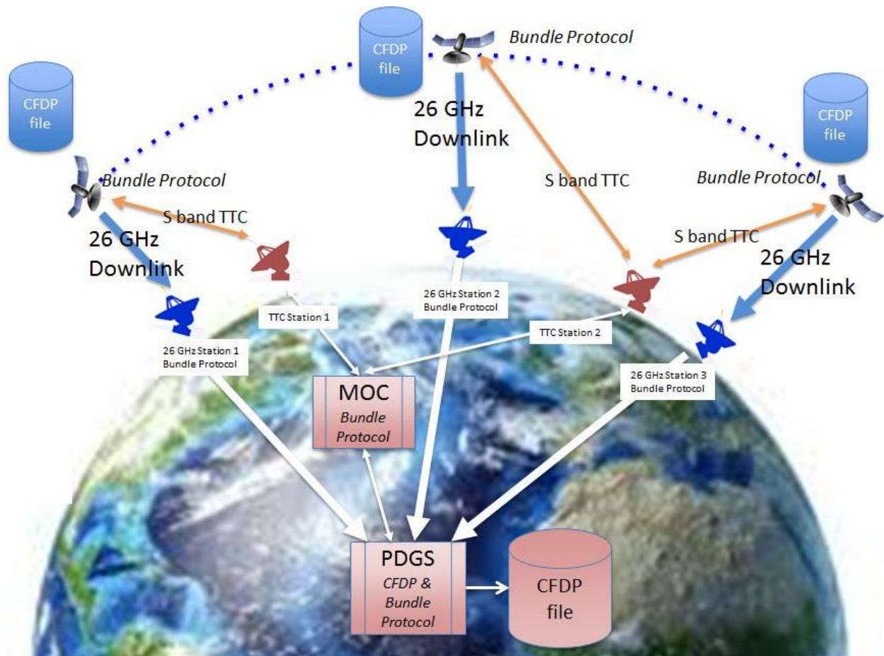
Figure I-2. Internetworking Using DTN Architecture. Different TTC Stations Close the BP at S-band when Overlapping with 26 GHz. TTC Stations Need to be Collocated with Receiving 26 GHz Stations for ACM.
