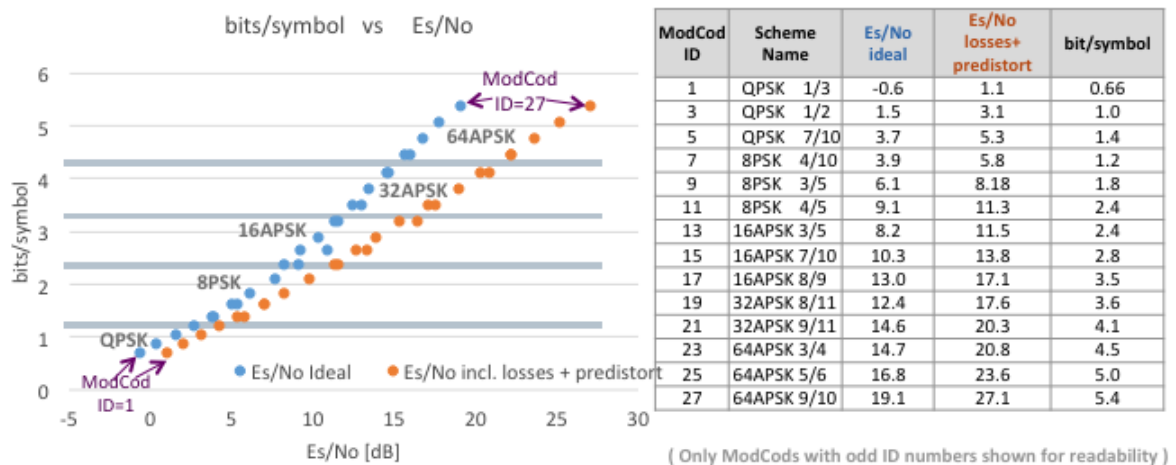
Figure G-1. Data Rate over SNR/bit for 27 ModCods
