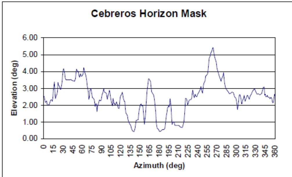
Figure F-2. Cebreros Horizon Mask
