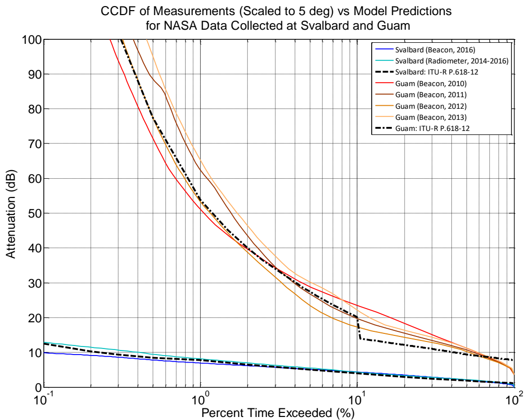
Figure H-2. CCDF of NASA measurements taken in Svalbard (arctic region) and Guam (tropical region), scaled to 5 deg elevation angle and compared with ITU models.
