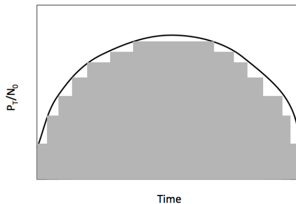
Figure 3-2. Link Budget with Advanced Coding and Modulation Techniques
